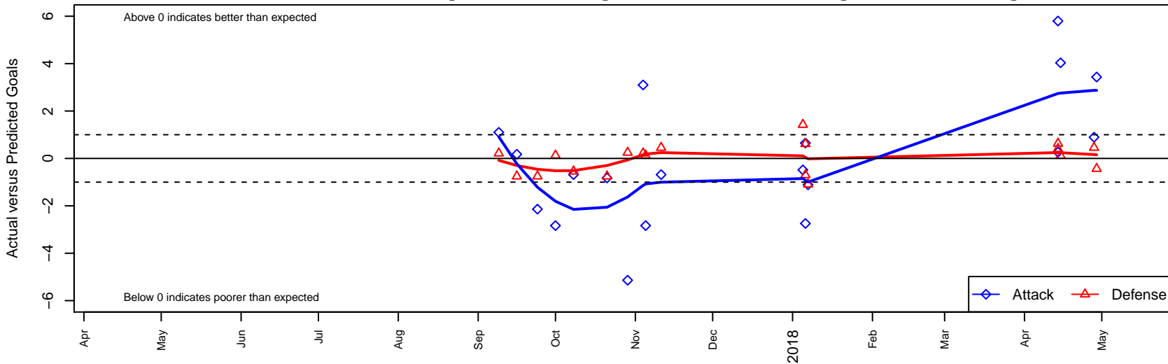
Liga Tlaxtli FC Guerreros B05 Dots are actual minus expected GF (blue circles) and GA (red triangles). Blue line is smoothed change in attack strength. Red is smoothed change in defense strength.
